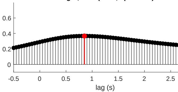
dLight, dark (n=25, opt=0.85s)
