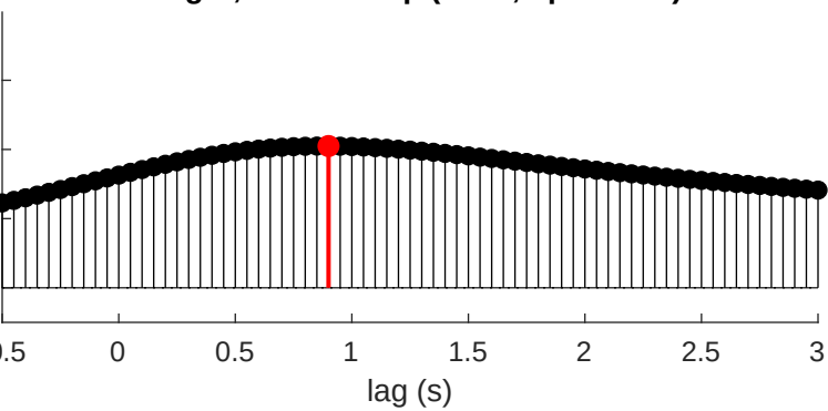
dLight, closed loop (n=71, opt=0.90s)
