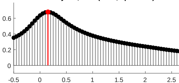
GRAB(DA2m), dark (n=19, opt=0.55s)
