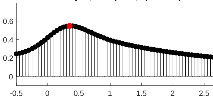
syt7f, dark (n=21, opt=0.35s)
