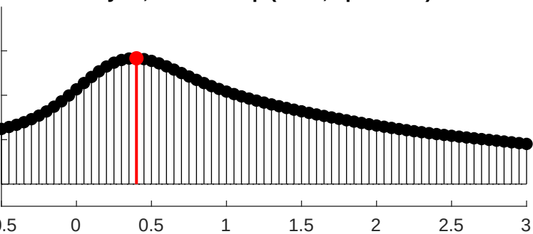
syt7f, closed loop (n=27, opt=0.40s)
